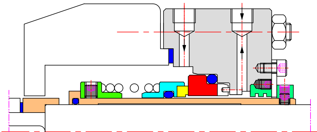
80 SERIES SINGLE SPRING MECHANICAL SEAL TYPE 8201 CARTRIDGE ARRANGEMENT WITH DIFFERENT API PLAN 11& 62
